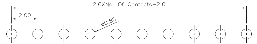
Recommended P.C.B. Layout
