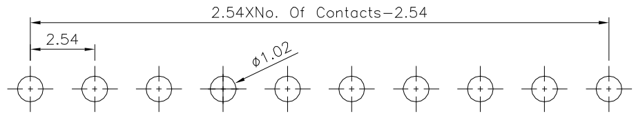
⚠ Recommended P.C.B. Layout(Top View) (PCB Board Tolerance±0.05)
