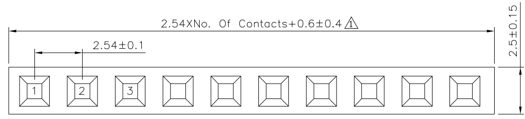
⚠ Recommended P.C.B. Layout(Top View) (PCB Board Tolerance±0.05)
