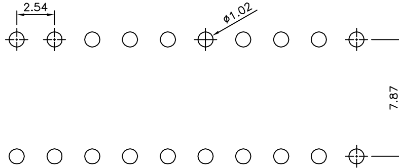
Recommended P.C.B. Layout(Top View) (PCB Board Tolerance±0.05)
