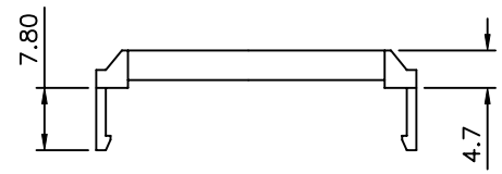
Strain Relief
