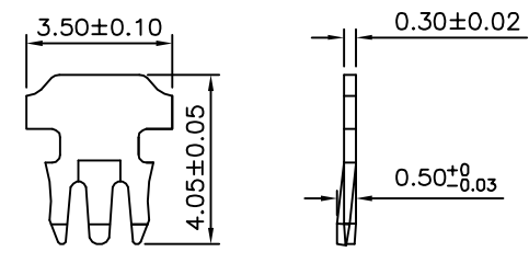
△ 3 Prongs For Solid Wire
