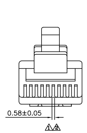
△ 2 Prongs For Stranded Wire
