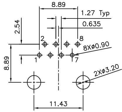
△ Recommended P.C.B. Layout Recommended P.C.B. Thickness:1.6mm Tolerance±0.05 (Top View)
