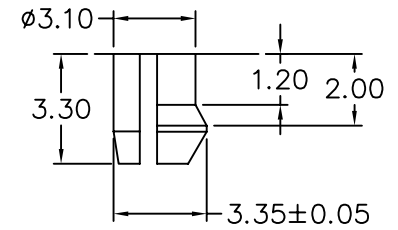
Detail X
