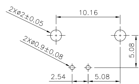
Recommended P.C.Board Layout Without Mounting Posts
