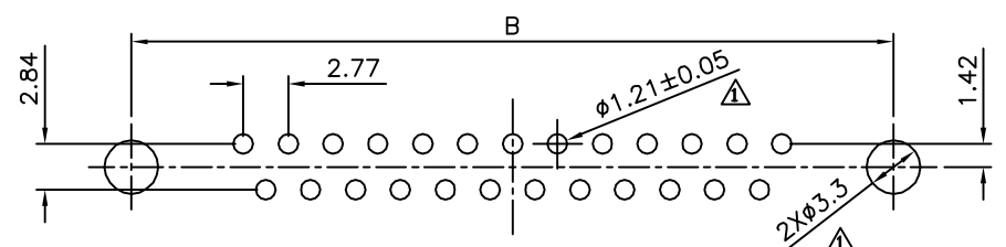
Recommended P.C.B. Layout △ PCB Thickness:2.00;Tolerance±0.05
