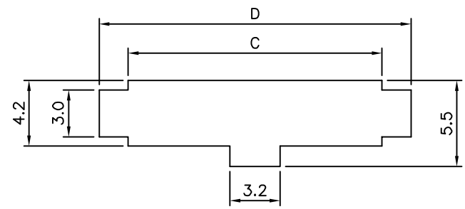
Panel Hole Dimensions
