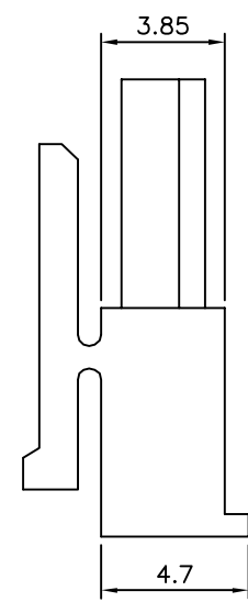
2 Pin
