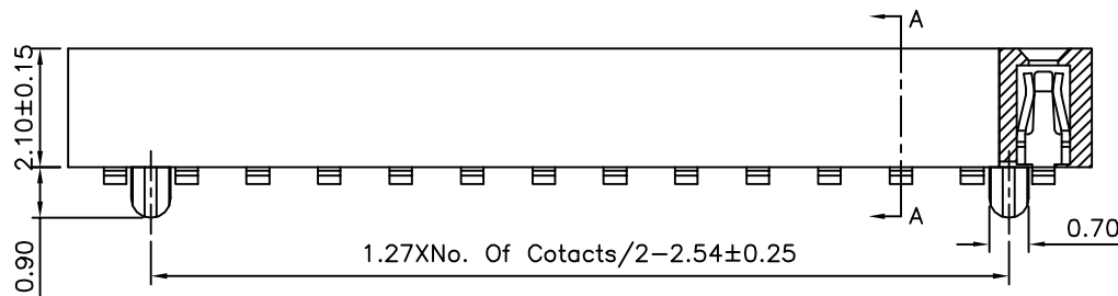
Section B-B
