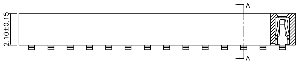
Section B-B
