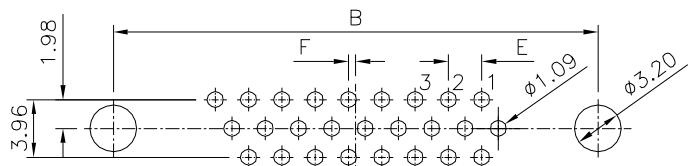
Recommended P.C.B. Layout(26,44,62 Pin)
