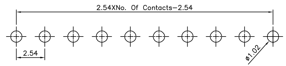
Recommended P.C.B. Layout PCB Board Tolerance±0.05(Top View)
