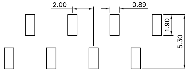
Recommended P.C.B. Layout Standard Layout
