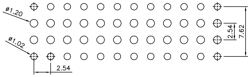
▲ Recommended P.C.B Layout(Top Side) ▲ PCB Board Tolerance±0.05
