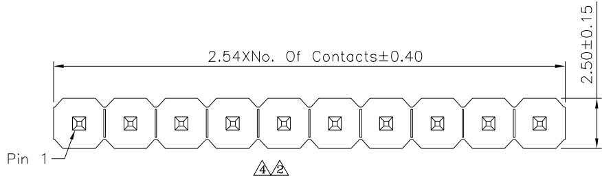
△4 Recommended P.C.B. Layout
