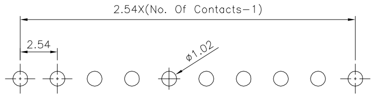
△4 Recommended P.C.B. Layout
