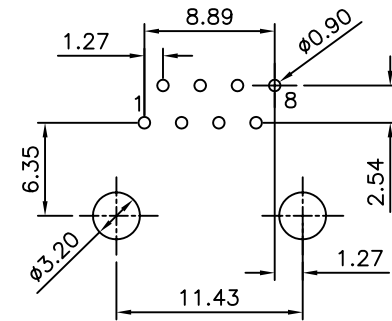
PC Board Layout Ref.
