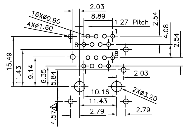
Recommended P.C.B. Layout (Top View) △ (PCB Board Tolerance±0.05) Thickness:1.6mm
