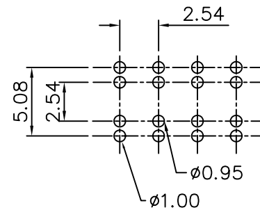
P.C. Board Hole Layout
