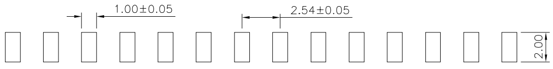
Recommended P.C.B. Layout Tolerance:±0.05
