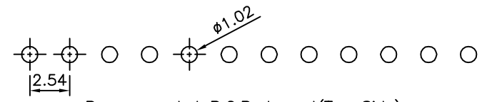
Recommended P.C.B. Layout (Top Side) (PCB Board Tolerance ±0.05)
