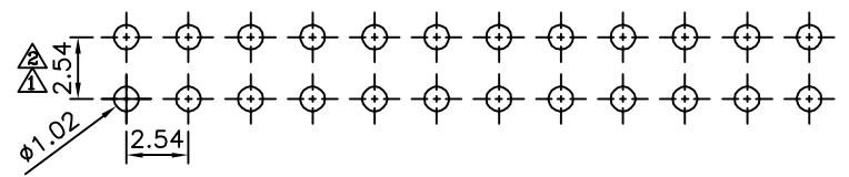
Recommended P.C.B. Layout(Top Side) (PCB Board Tolerance±0.05)
