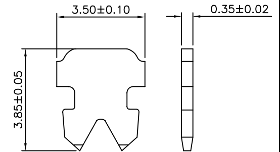
2 Prongs For Stranded Wire
