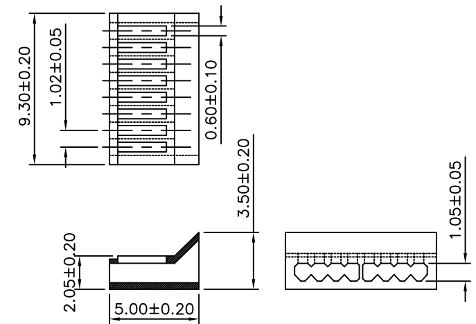
2 Prongs For Stranded Wire
