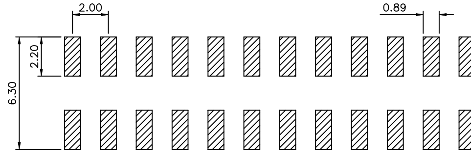
Recommended P.C.B. Layout(Top Side) (PCB Board Tolerance±0.05)
