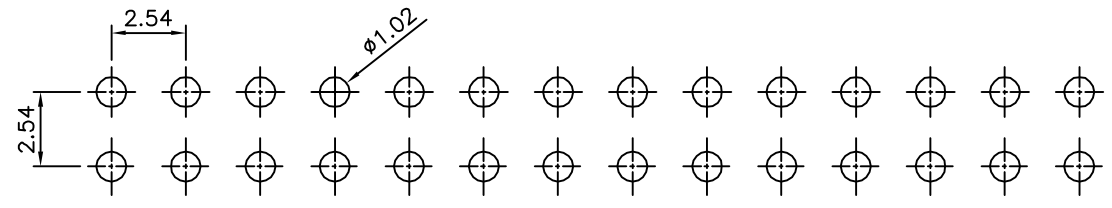
Recommended P.C.B. Layout(Top Side) (PCB Board Tolerance±0.05)
