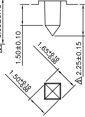
Detail K
