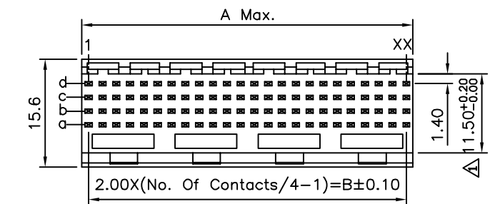
Recommended P.C.B. Layout (PCB Board Tolerance±0.05)
