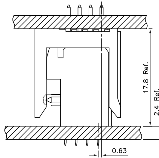
△ Board To Board Offset Application Example
