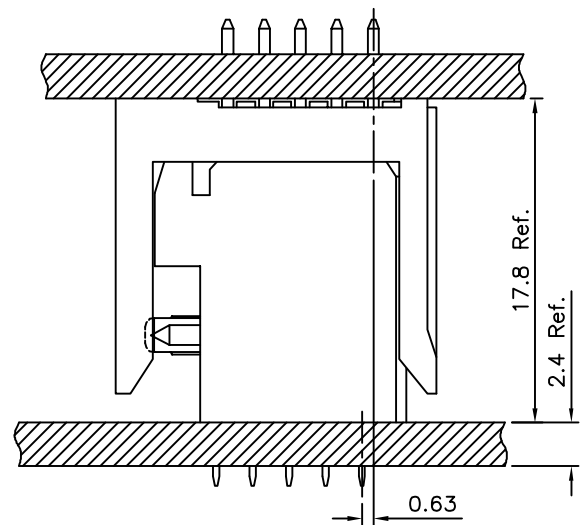
Board To Board Offset Application Example
