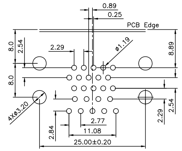
Recommended P.C.B. Layout (PCB Board Tolerance ±0.1)
