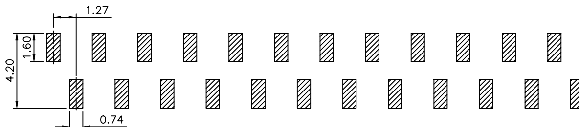
Recommended P.C.B. Layout (PCB Board Tolerance±0.05)
