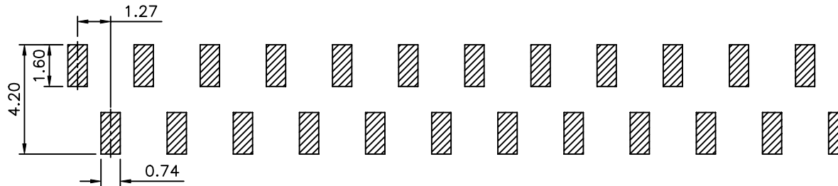
Recommended P.C.B. Layout (PCB Board Tolerance \pm 0.05 )
