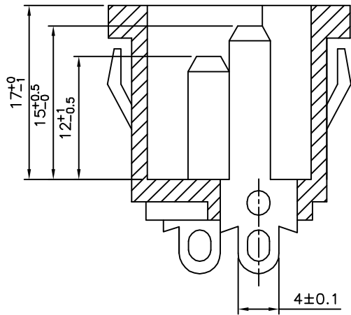
Panel Cutout Thickness 0.8mm~1.5mm
