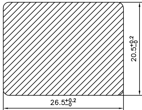
Panel Cutout Thickness 0.8mm~1.5mm
