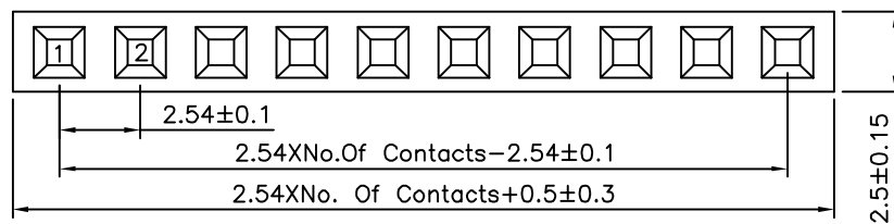
Recommended P.C.B. Layout(Top View) (PCB Board Tolerance±0.05)
