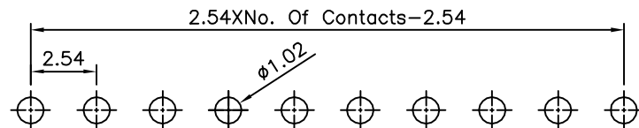
Recommended P.C.B. Layout(Top View) (PCB Board Tolerance±0.05)
