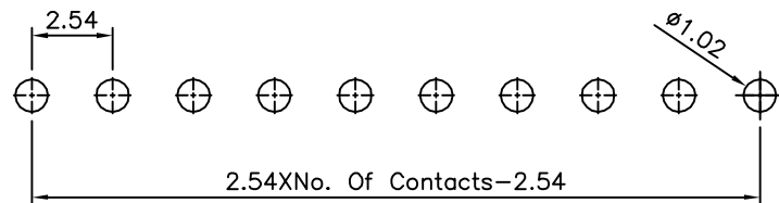
Recommended P.C.B. Layout(Top View) (PCB Board Tolerance \pm 0.05 )
