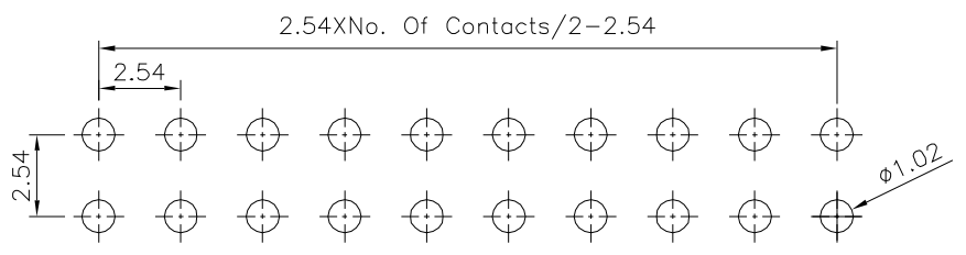
Recommended P.C.B. Layout (Top View) (PCB Board Tolerance ±0.05)
