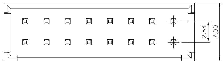
Recommended P.C.B. Layout (PCB Board Tolerance ±0.05)
