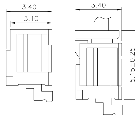
Mating Height Drawing
