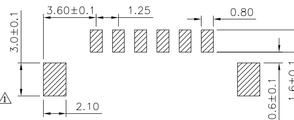
Recommended P.C.B. Layout(Top View) (PCB Board Tolerance±0.05)
