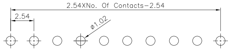
Recommended P.C.B. Layout(Top View) (PCB Board Tolerance±0.05)
