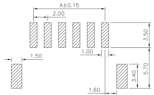
Recommended P.C.B. Layout (PCB Board Tolerance±0.05)
