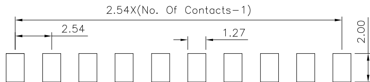
Recommended P.C.B. Layout
