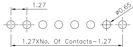
⚠ Recommended P.C.B. Layout(Top View) (PCB Board Tolerance \pm 0.05 )
