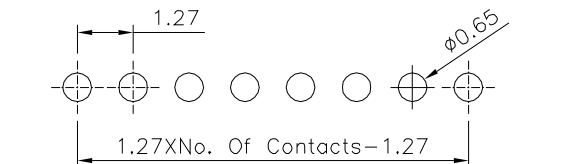
⚠ Recommended P.C.B. Layout(Top View) (PCB Board Tolerance \pm 0.05 )
