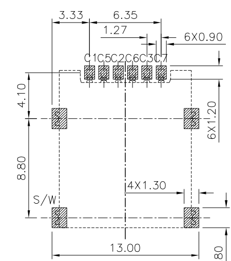
Recommended P.C.B. Layout (PCB Board Tolerance ±0.05) ▨ SMT Solder Area
