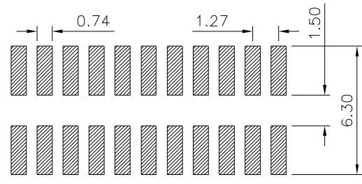
Recommended P.C.B. Layout (PCB Board Tolerance ± 0.05)
