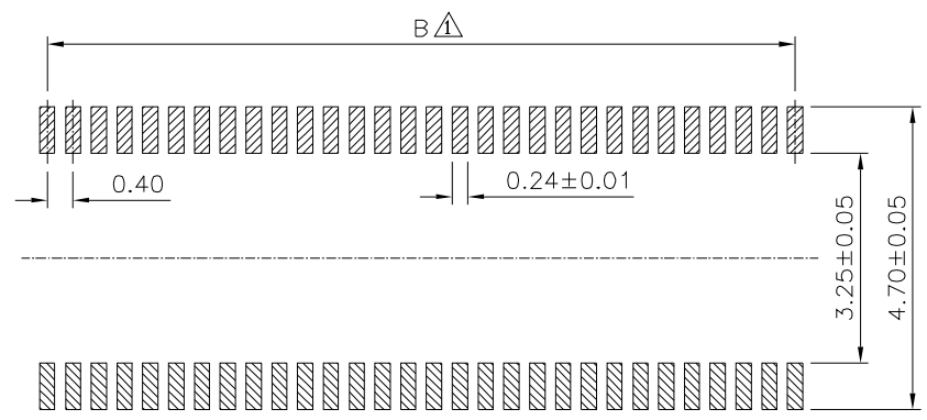
Recommended P.C.B. Layout (PCB Board Tolerance±0.03)
