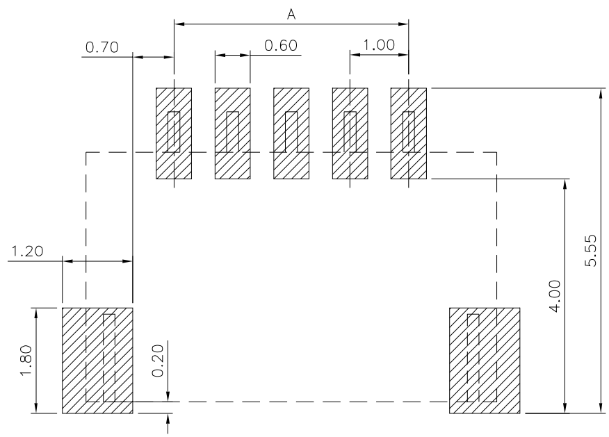
Recommended P.C.B. Layout Total Tolerance±0.05
