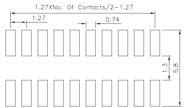
Recommended P.C.B. Layout Tolerance:±0.05(Top View)
