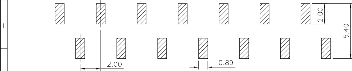
Recommended P.C.B. Layout(Top Side) (PCB Board Tolerance±0.05)
